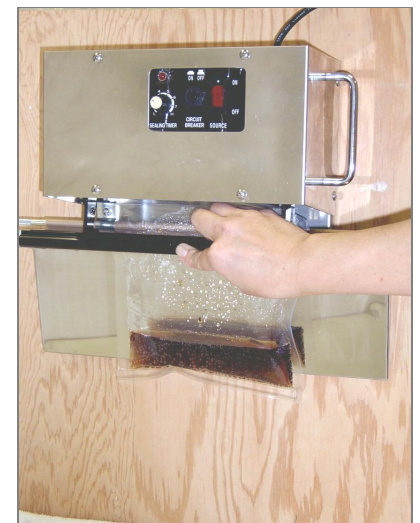
Sealing liquid with vertical sealing.
